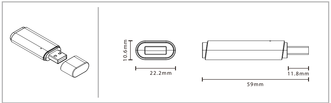
USB Repeater
