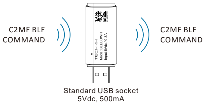
USB Repeater
